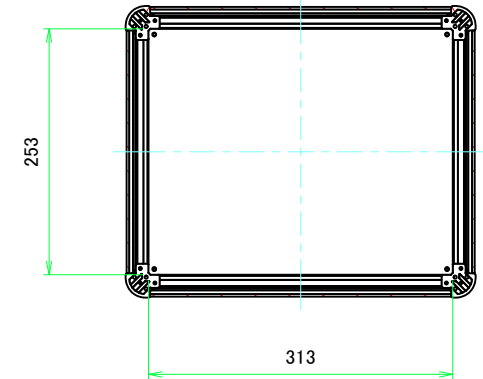
C-C (1:5.5)
